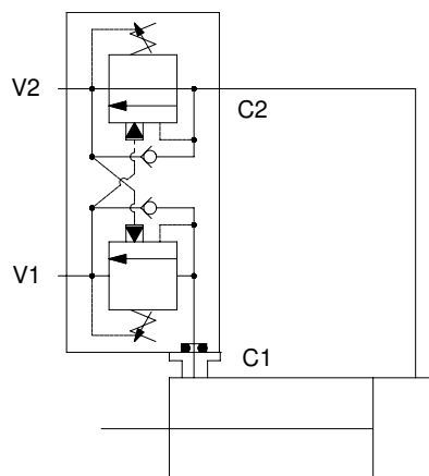
Double Counterbalance, Head Mounted
