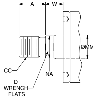
Thread Style 8 (NFPA Style IM) Intermediate Male
