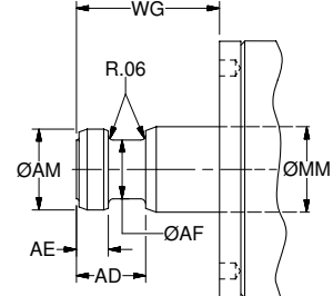
Style 55 2 Flanged Rod End
