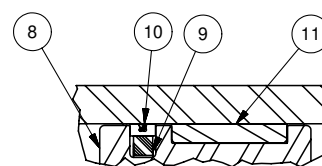
Optional Mixed Media Piston
