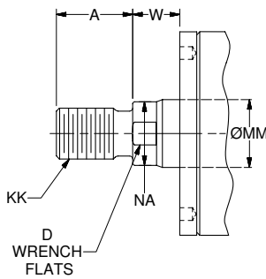
Thread Style 4 (NFPA Style SM) Small Male
