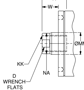
Thread Style 9 1 (NFPA Style SF) Small Female
