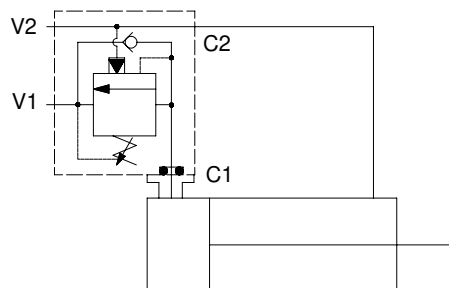
Single Counterbalance, Cap Mounted
