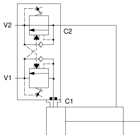
Double Counterbalance, Cap Mounted
