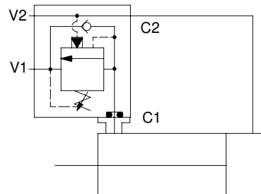
Single Counterbalance, Head Mounted
